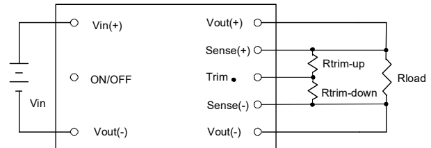
Output Voltage Trim Circuit Configuration
