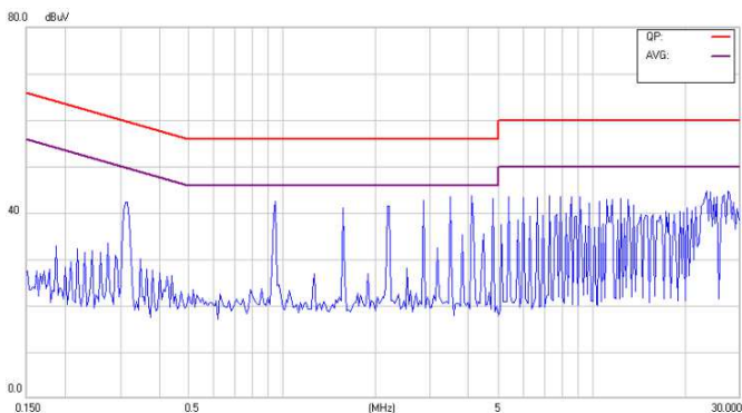
Conducted Class B of CHB350-24S3V3
