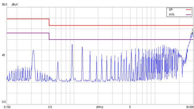
Conducted Class A of CHB350-24S28
