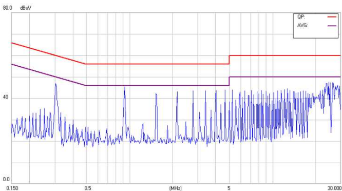
Conducted Class B of CHB350-24S05
