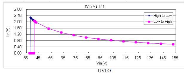
CQB100W-110SXX I in Vs V in
