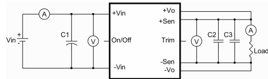
CQB100W-110S series Test Setup
