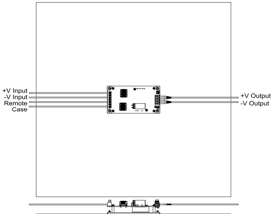
Figure 2 CQB150-300SXX-CMFC with Heat Sink Aluminum Plate (17x17x0.04 inch)
