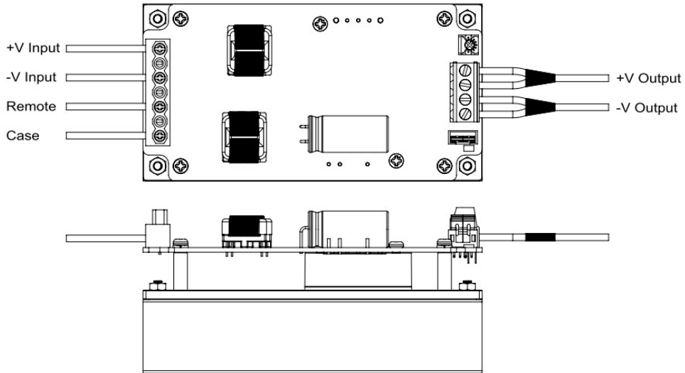
Figure 1 CQB150-300SXX-CMFC with Heat Sink FBL254
