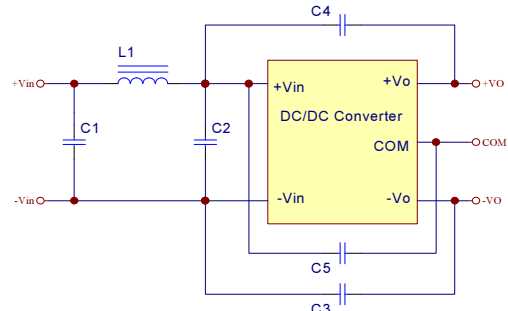
EC4SAWH dual output module
