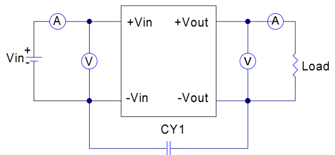
EC4SAWH Series Test Setup
